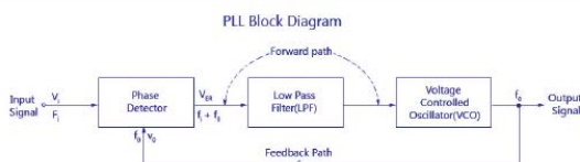
Block Diagram – Phase Locked Loops
