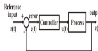
Closed Loop SISO System
