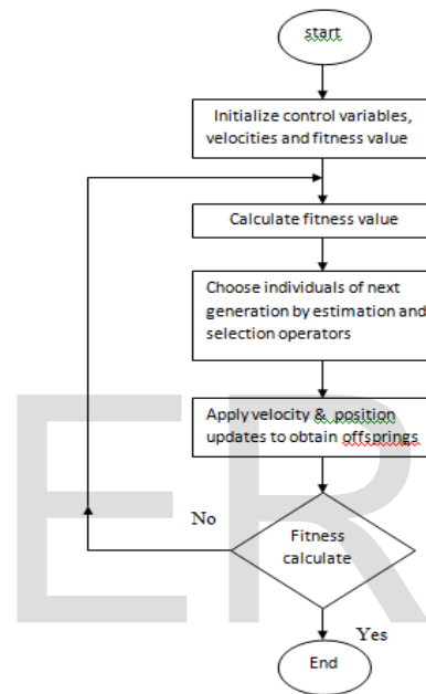
Flowchart of PSO
