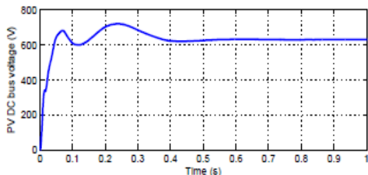
Response of the DC voltage in PV system
